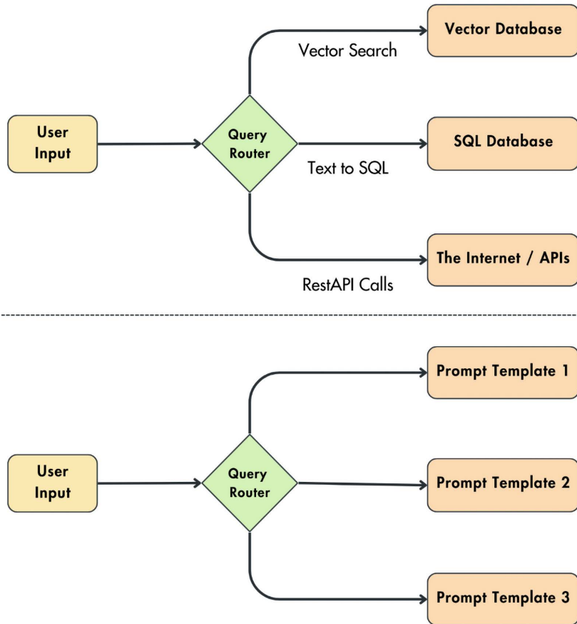
Figure 4.6: Query routing
